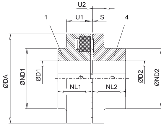
Figure A-4 Type BDS
